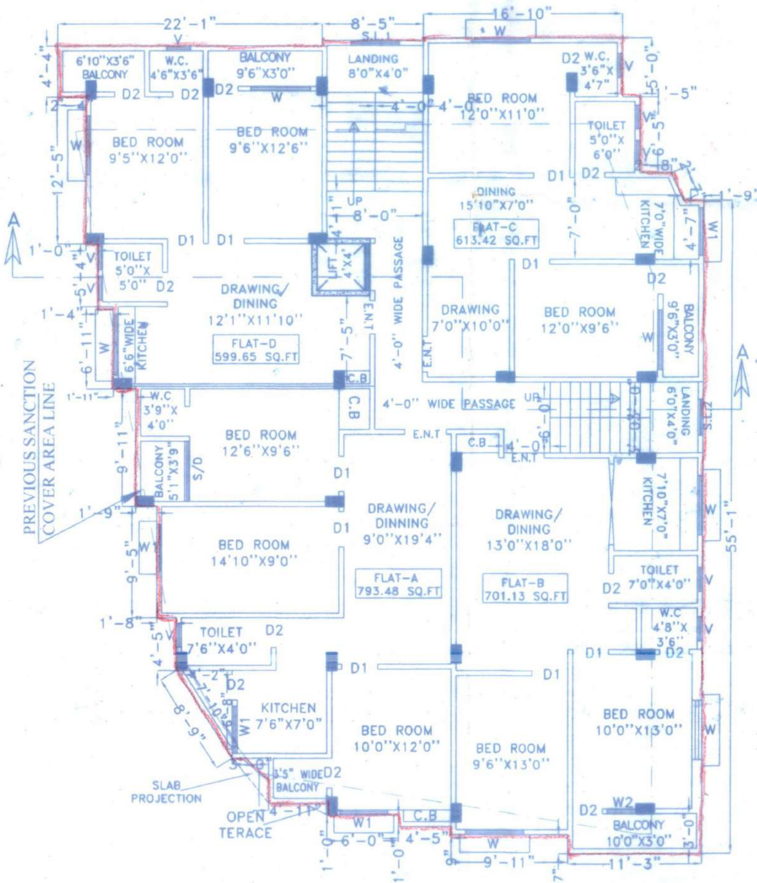
REVISED FIRST FLOOR PLAN
