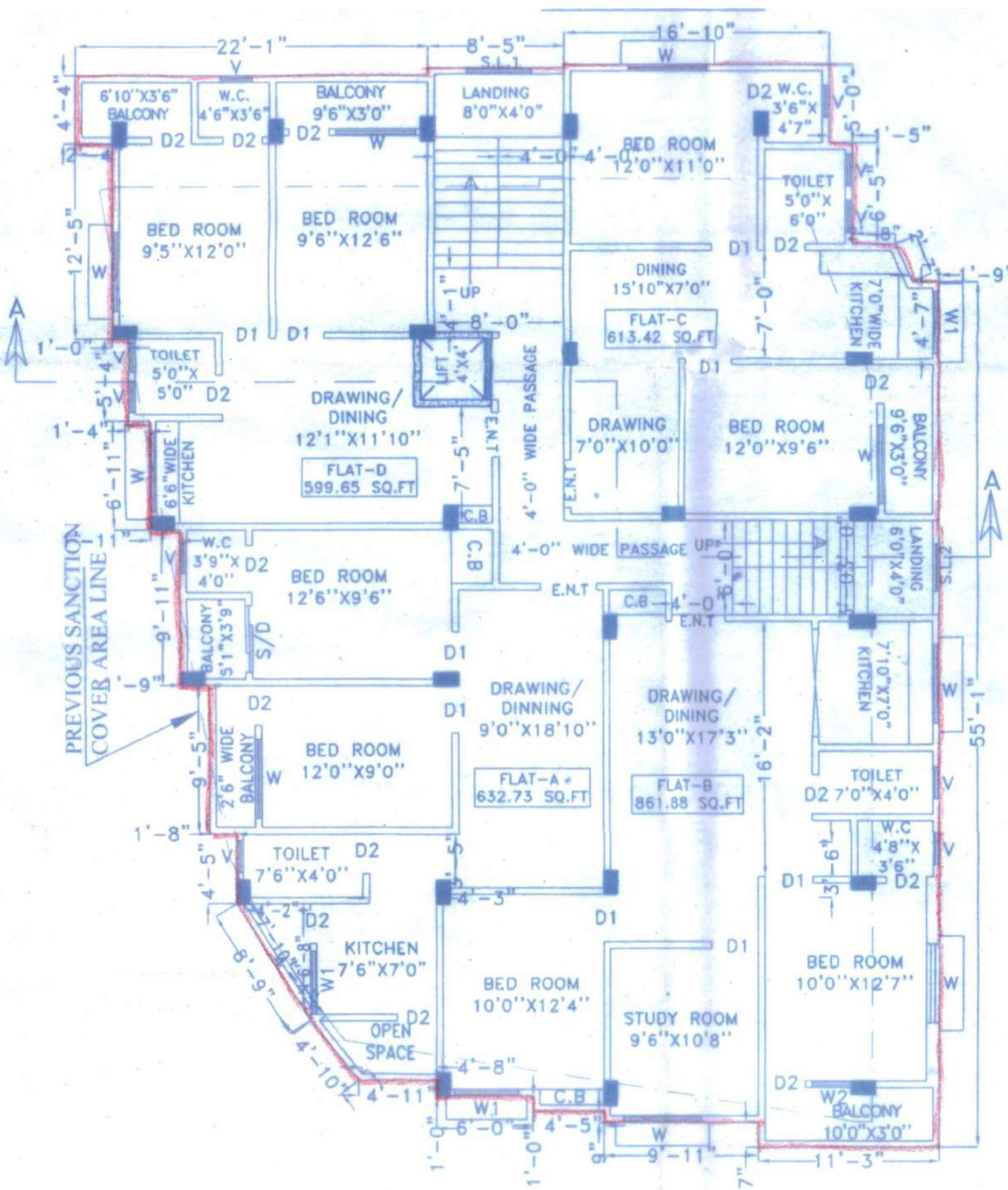
REVISED THIRD FLOOR PLAN
